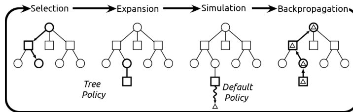
Fig. 1: Steps of the Monte Carlo Tree Search.
